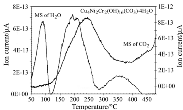
Fig. 2 Examples of the MS of water and carbon dioxide for the hydrotalcites (\text{Ni}_x\text{Cu}_{6-x})\text{Cr}_2(\text{OH})_{16}(\text{CO}_3)\cdot 4\text{H}_2\text{O}
