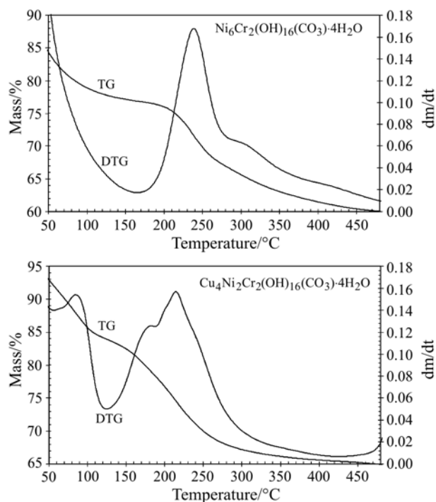
Fig. 1 Examples of the differential mass loss of hydrotalcites of formula (\text{Cu}_{6-x}\text{Ni}_x)\text{Cr}_2(\text{OH})_{16}(\text{CO}_3)\cdot 4\text{H}_2\text{O}
